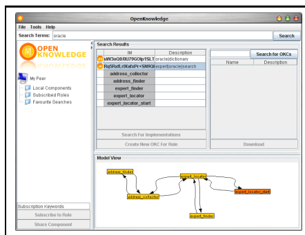
Fig. 16. Part of the Open Knowledge GUI
